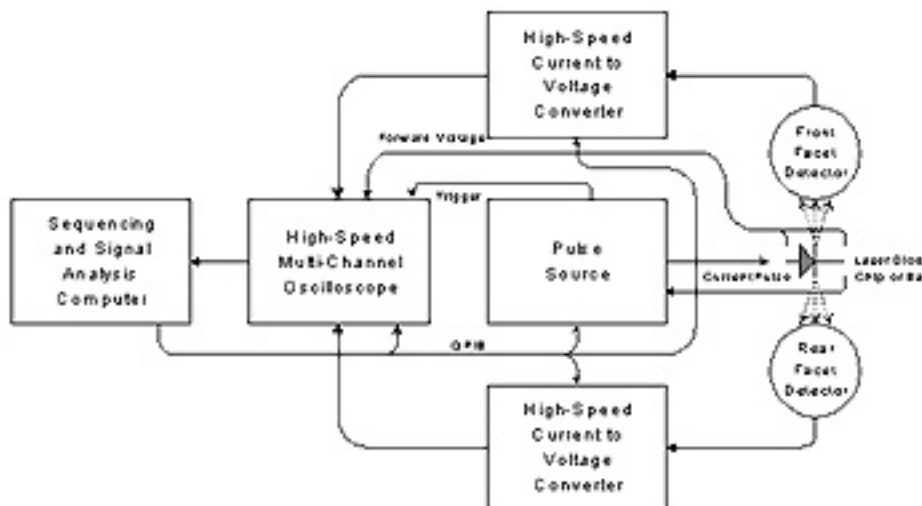
Figure 1. Second Generation Pulsed L-I-V Test System
